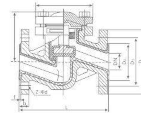
H41 F 型法兰连接止回阀(直通升降式) H41-F 46 Flange connection valve (straight-through lift)
